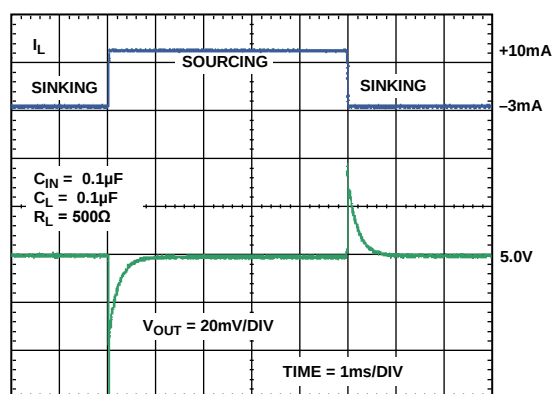
Figure 29. ADR3550 Load Transient Response
