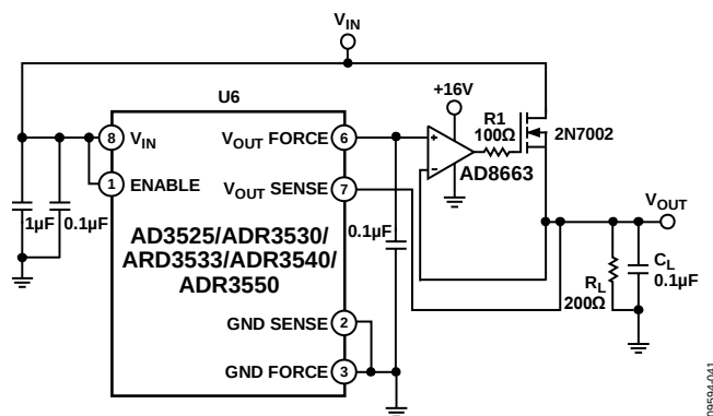
Figure 41. Boosted Output Current Reference
