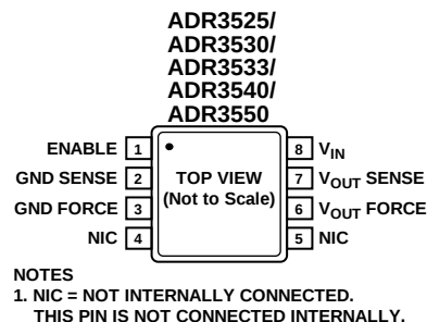
Figure 1. 8-Lead MSOP (RM-8 Suffix)
